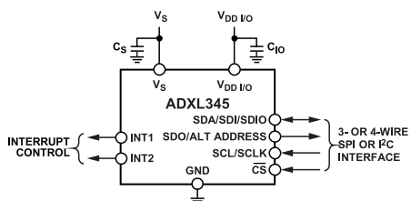
Figure 44. Application Diagram
